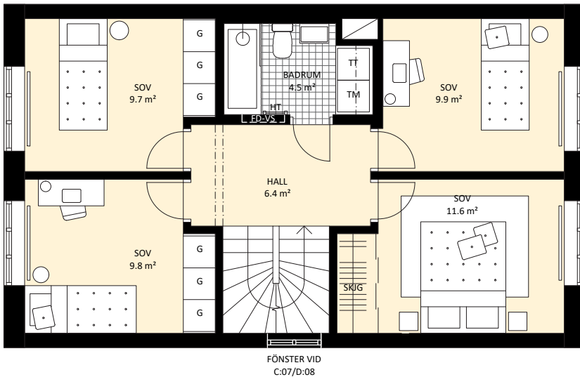
PLAN 1
